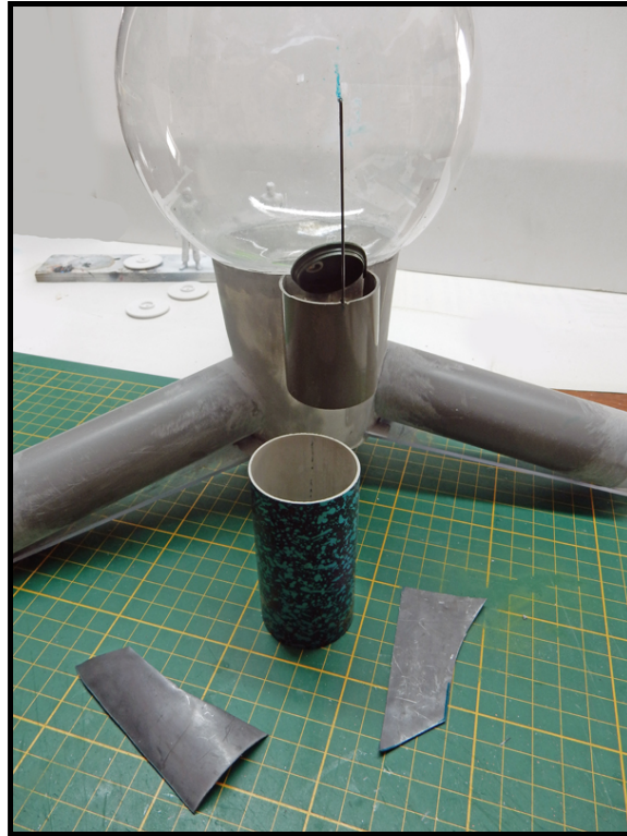
Securing the airlock using a plastic cylinder and a sheet of lead...
