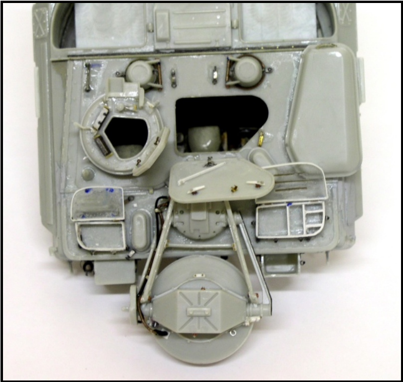
PHASE TWO: ASSEMBLING THE TURRET
