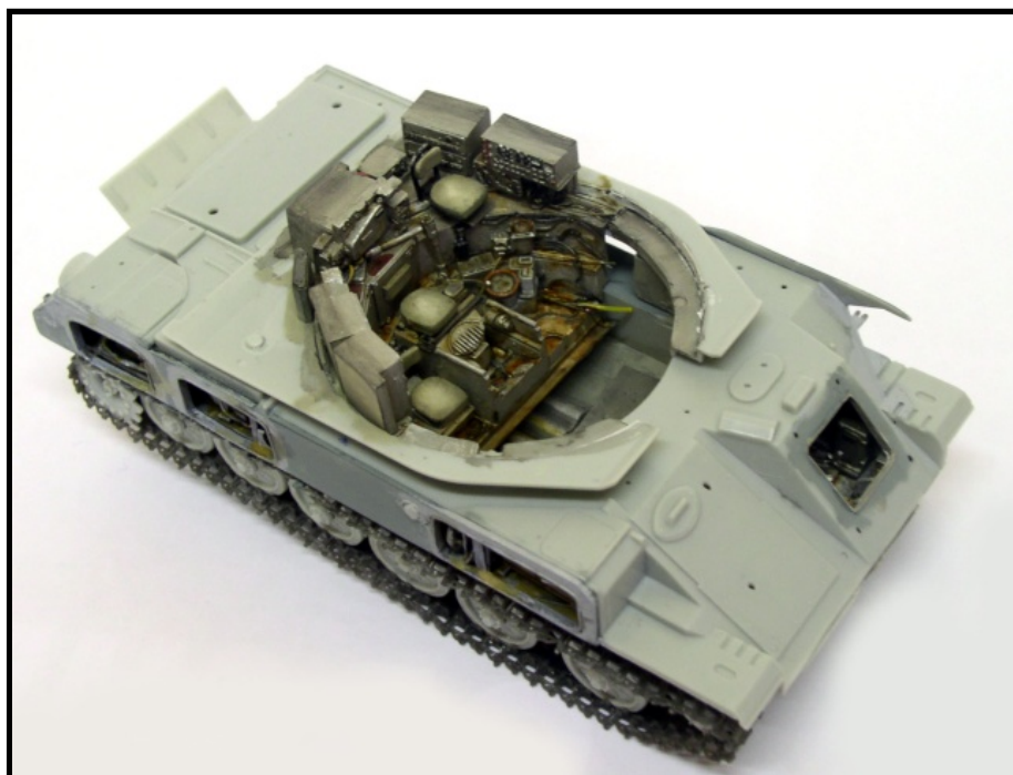
An overview of the resin kit in place...
